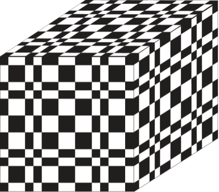
Thue–Morse cube
